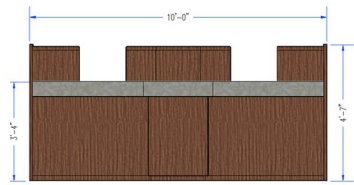
FRONT VIEW POD D
