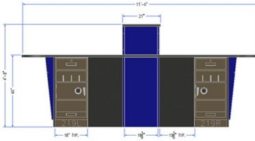
REAR VIEW POD B
