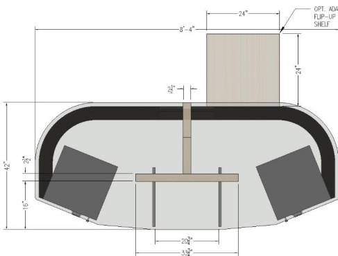
TOP VIEW POD C
