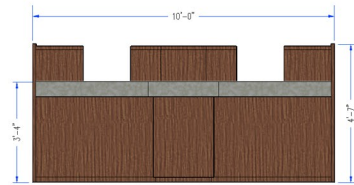
REAR VIEW POD D
