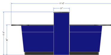
FRONT VIEW POD B
