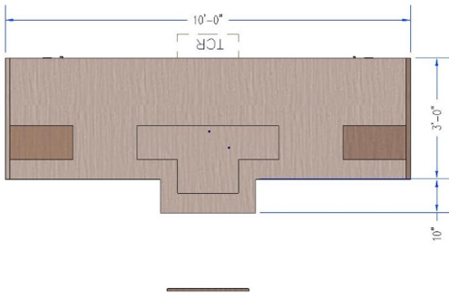
TOP VIEW POD D
