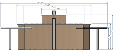
FRONT VIEW POD F
