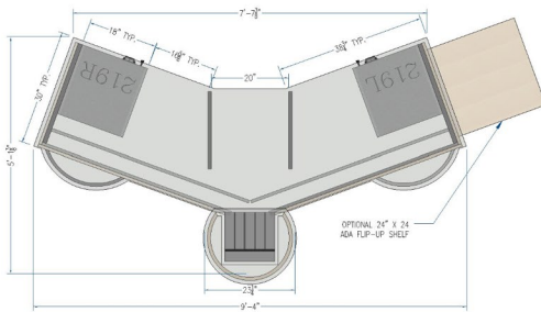
TOP VIEW POD A
