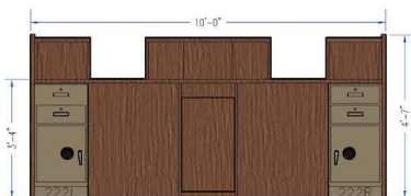
REAR VIEW POD D
