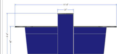
FRONT VIEW POD B
