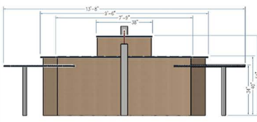
FRONT VIEW POD F
