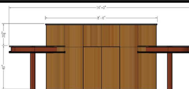
FRONT VIEW POD E
