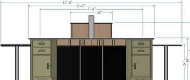
REAR VIEW POD F
