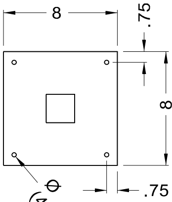
SLOPING INSERT WITH PAPER WEIGHT ( SECURED INSIDE )
